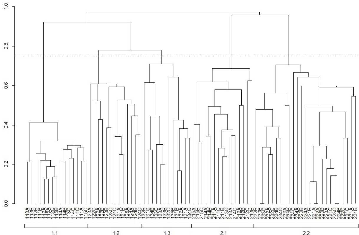
Fig. 3 - Dendrogram resulting from the cluster analysis of relevés. The dotted line indicates the dissimilarity value of 0,75.
