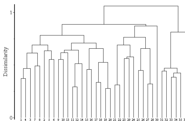
Fig. 2 - Dendrogram obtained through the synoptic comparison among the holm oak communities surveyed (cluster analysis, UPGMA). Ampelodesmo mauritanici-Quercetum ilicis ass. nova subass. typicum (branches 1-8; Tab. 9, rel. 1-8) and viburnetosum tini subass. nova (branches 9-20; Tab. 9, rel. 9-20); Sorbo torminalis-Quercetum ilicis ass. nova (branches 21-30; Tab. 10, rel. 1-10); Aceri campestris-Quercetum ilicis (branches 31-36; Tab. 11, column 1).
